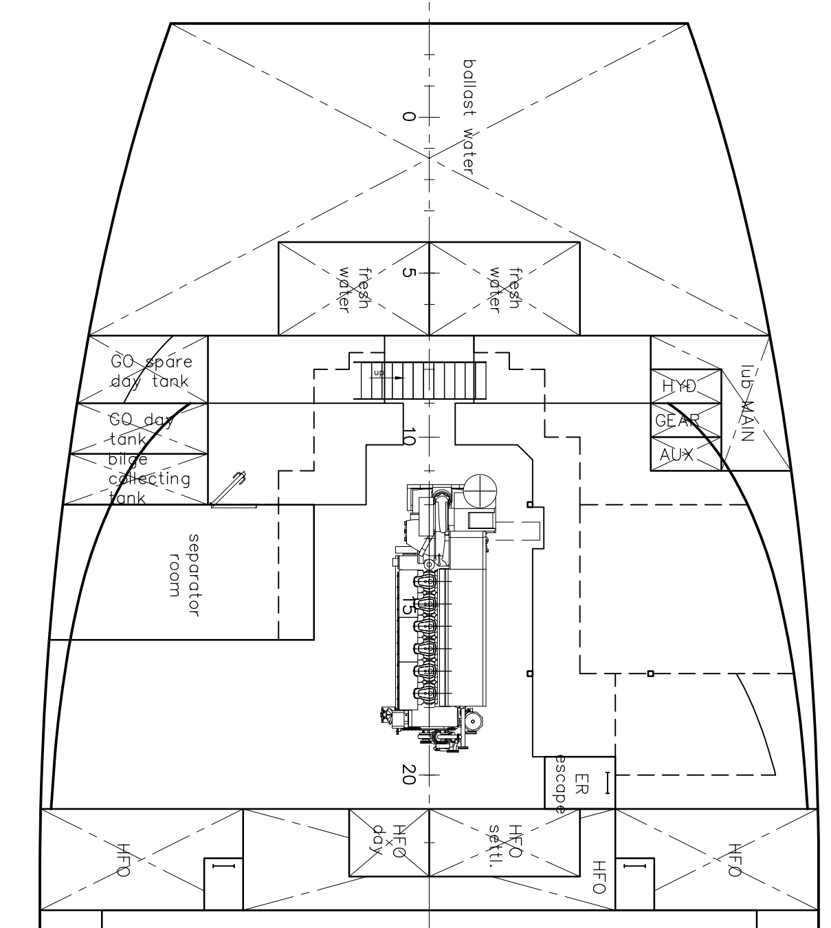
TWEENDECK ENGINE ROOM
