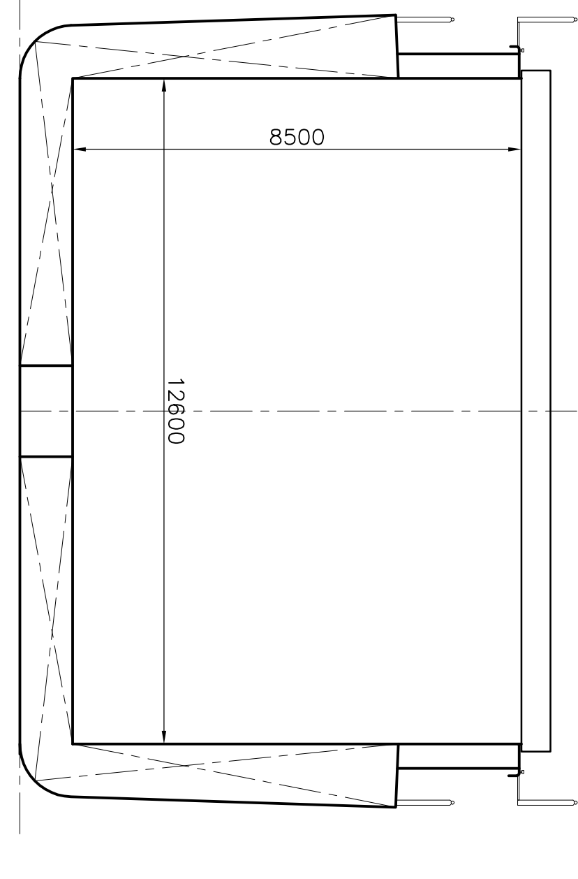
TWEENDECK ENGINE ROOM
