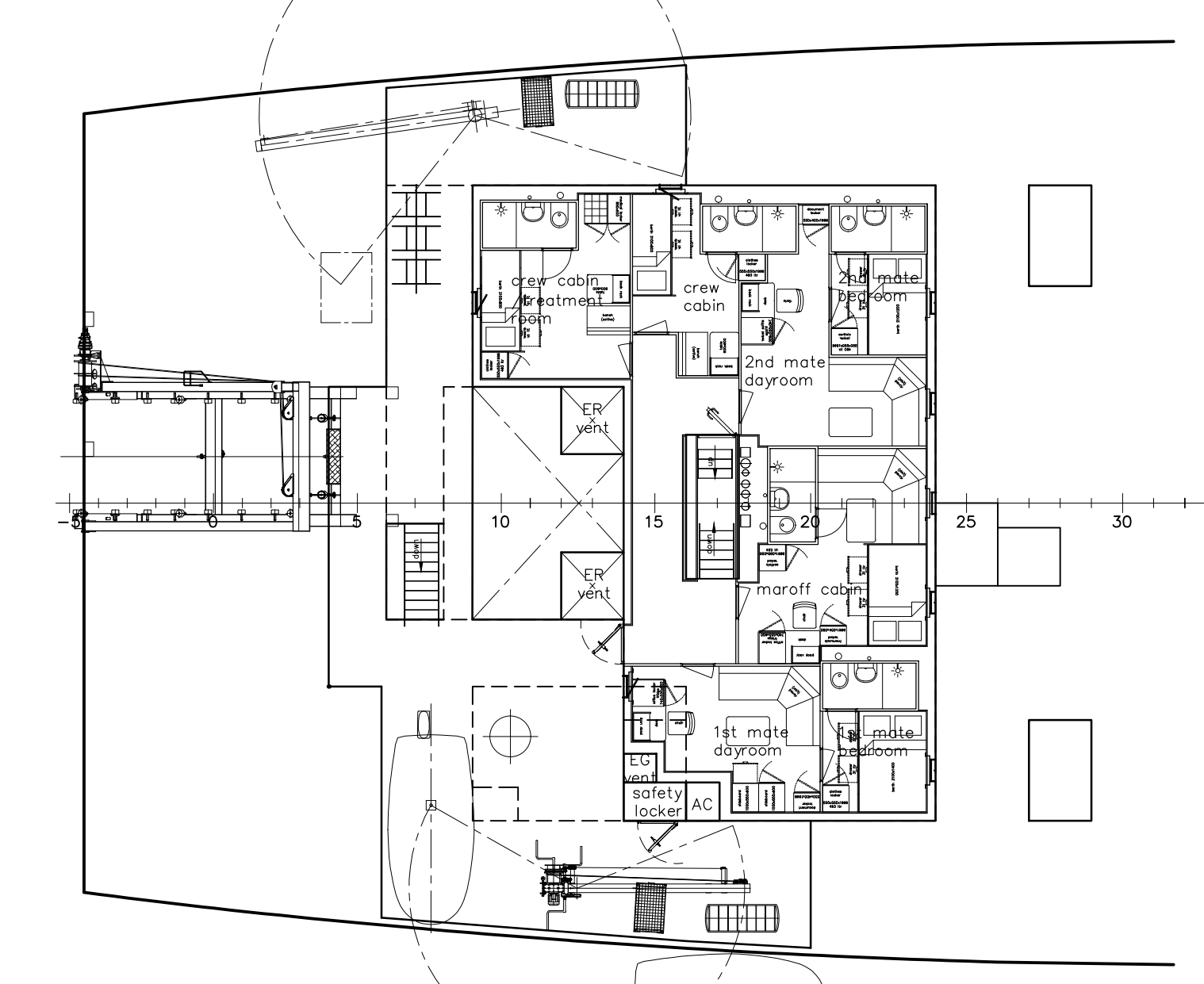
MAIN DECK
