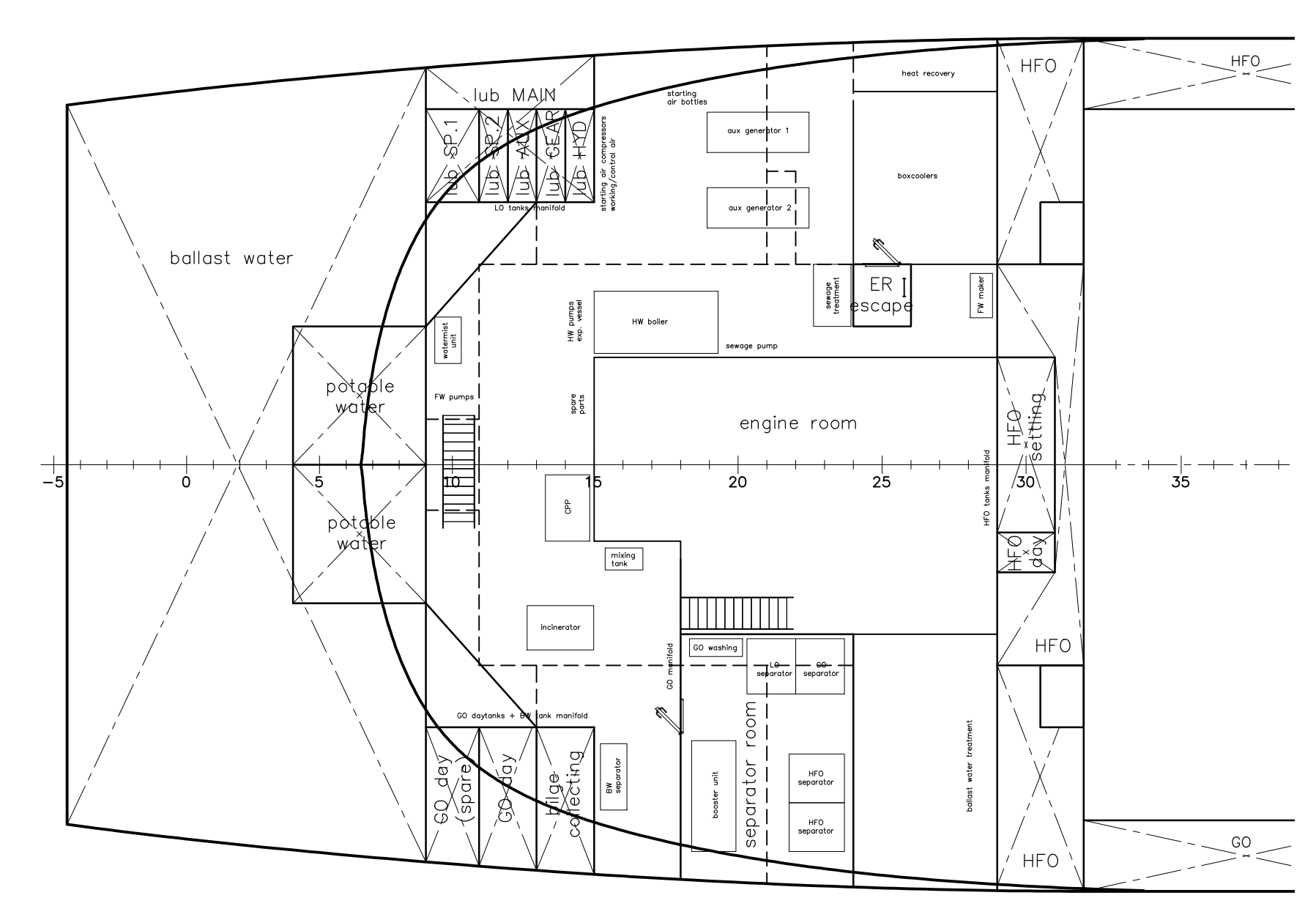
TWEENDECK ENGINE ROOM
