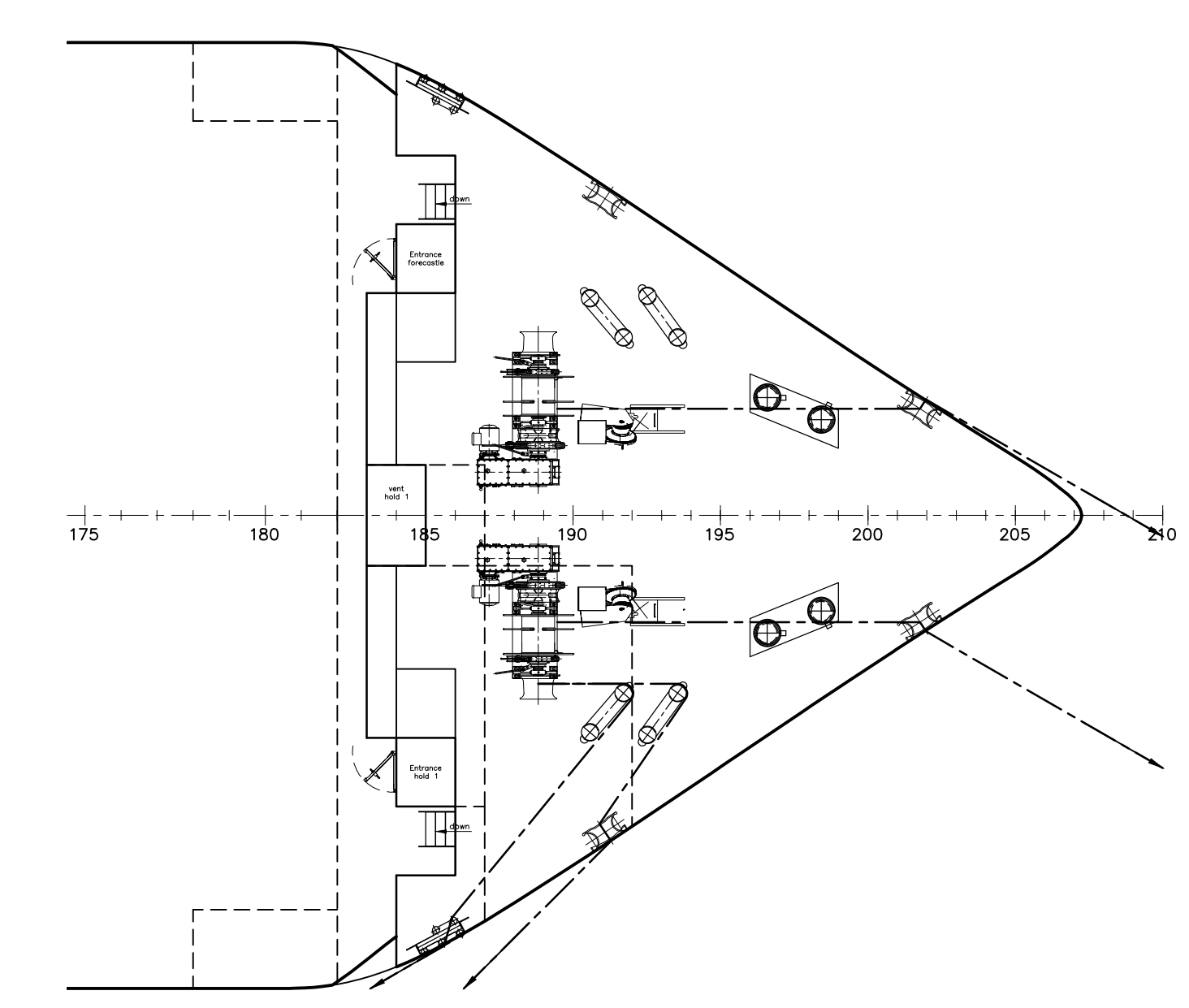
FORECASTLE DECK
