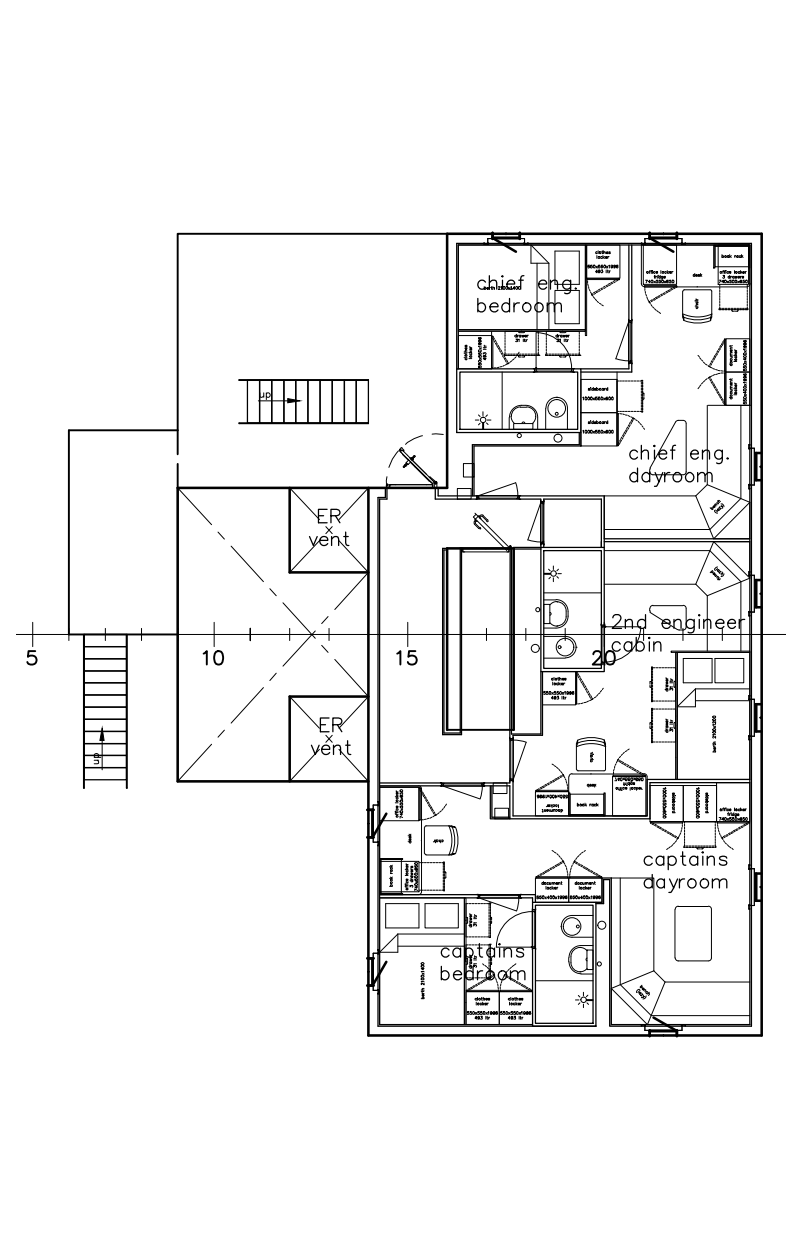
CAPTAINS DECK
